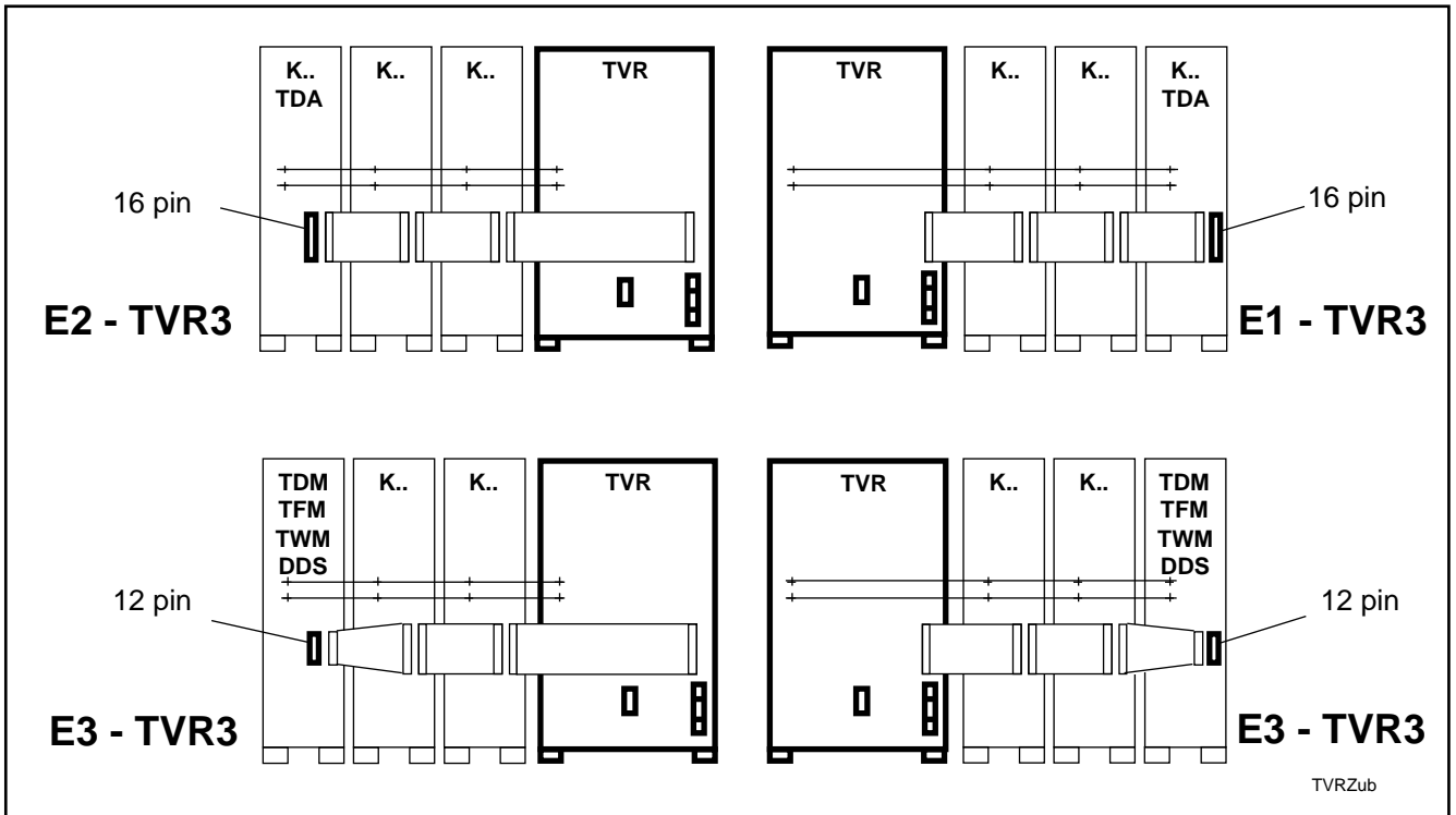
Fig. 8.2: Overview of electrical accessory kits
