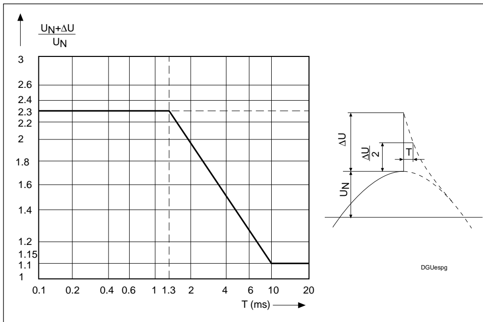
Fig. 3.6: Permissible non-periodic overvoltages as per VDE 0160
