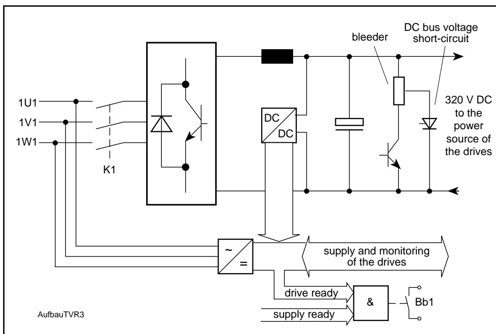
Figure1.2: TVR 3.1 - structure
